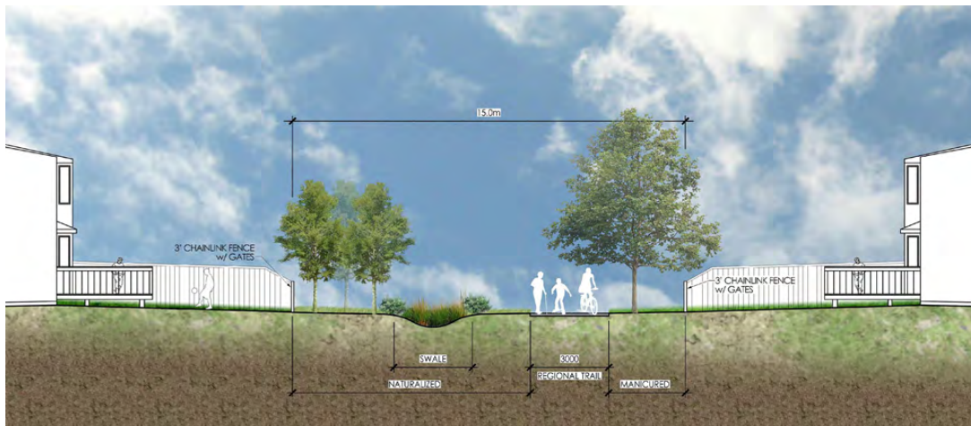
Section View 1:150
