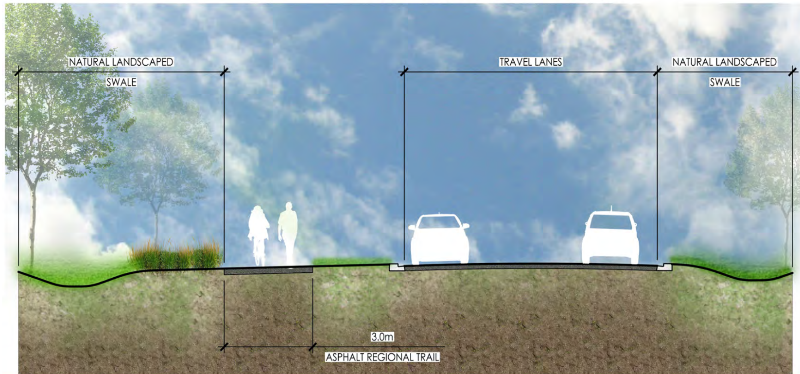
Figure 5.8 3.0m Asphalt – Reg. Blvd. Trail (F-F)
