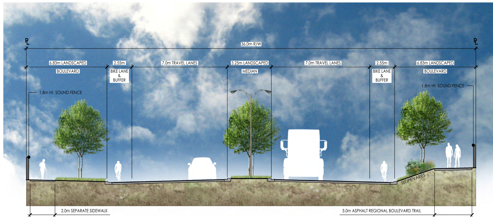
Figure 5.3 3.0m Asphalt – Regional Blvd. Trail – James Walker Trail (A-A)
