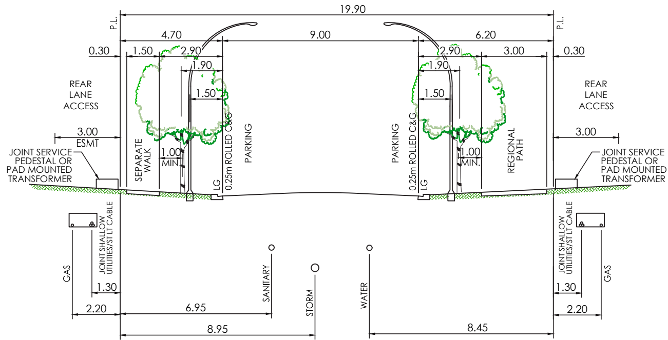
19.9m MODIFIED RESIDENTIAL PARKING BOTH SIDES / 2.0m SEPARATE WALK ONE SIDE / 3.0m REGIONAL PATH ONE SIDE
