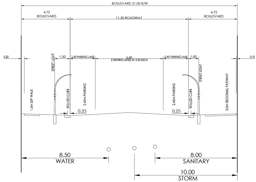
21.0m EXISTING RESIDENTIAL WILLOW DRIVE
