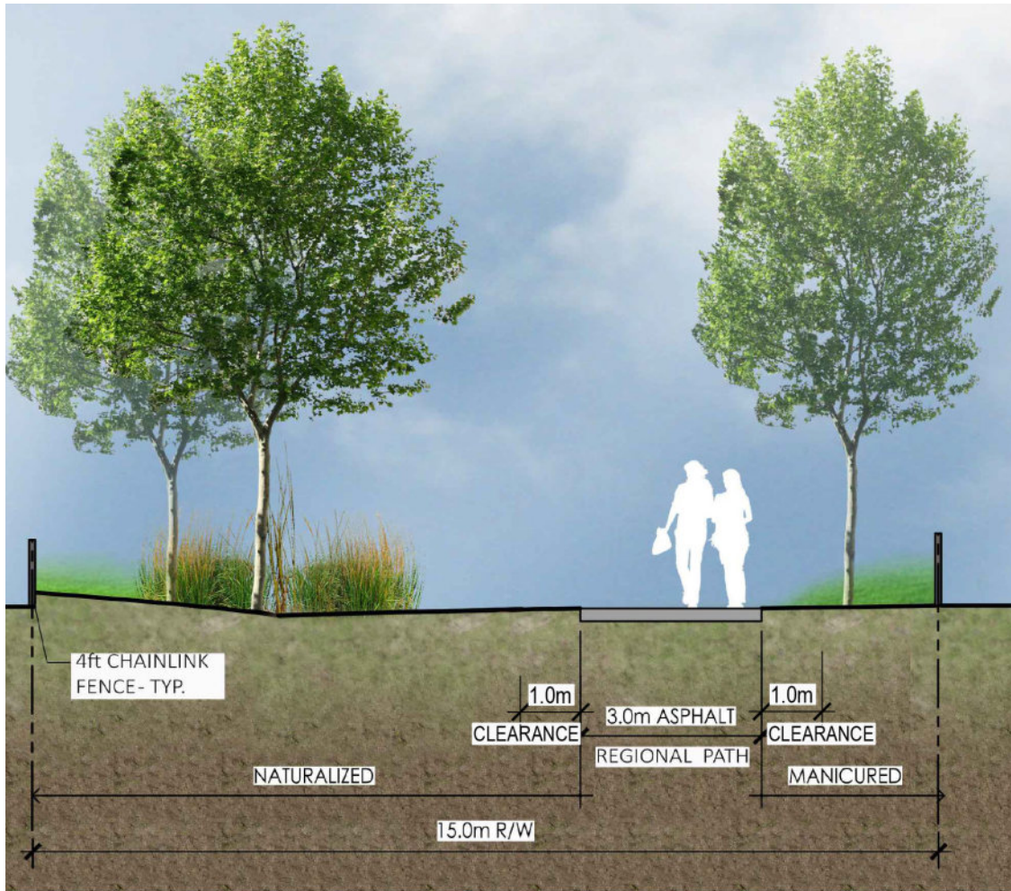
Figure 5.10 Linear Park - Regional Pathway (H-H)
