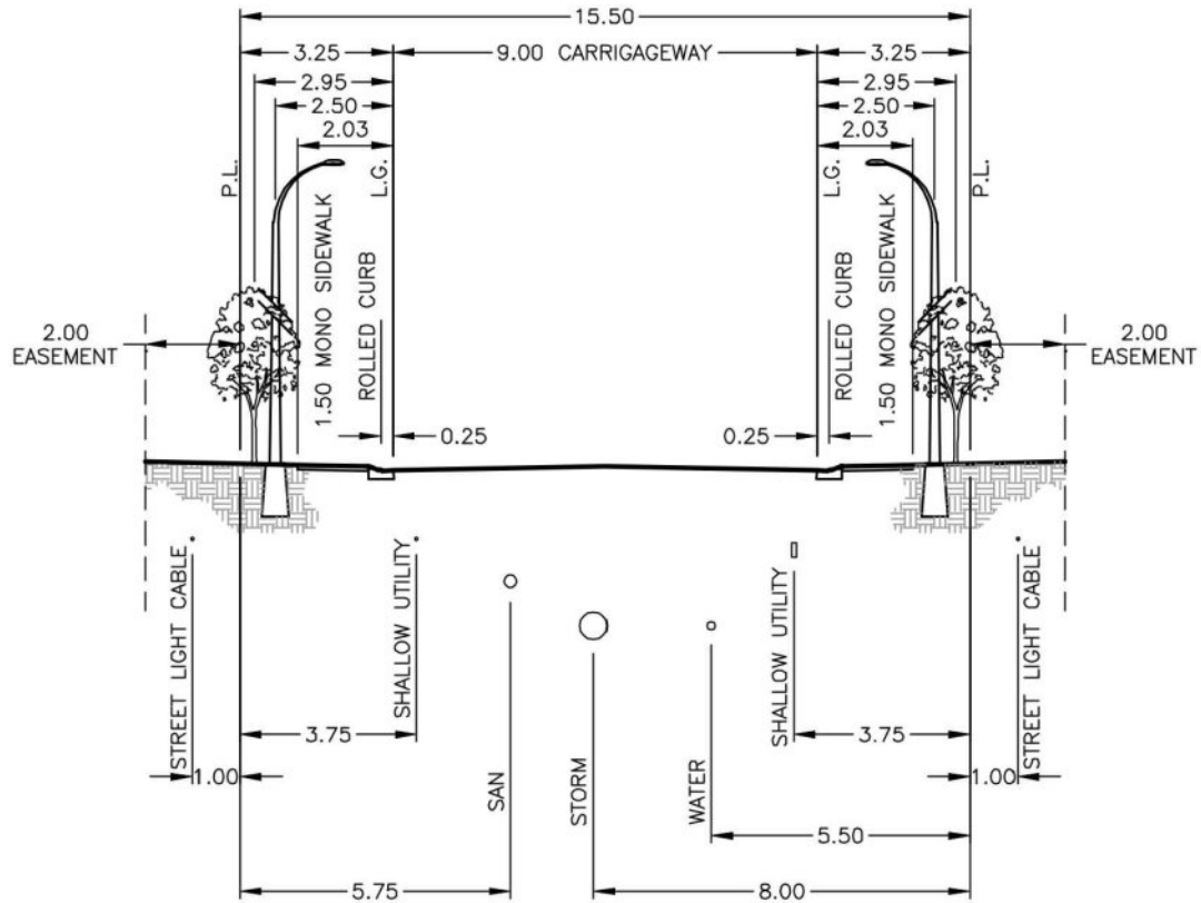
15.5m RESIDENTIAL w/ REAR LANE
