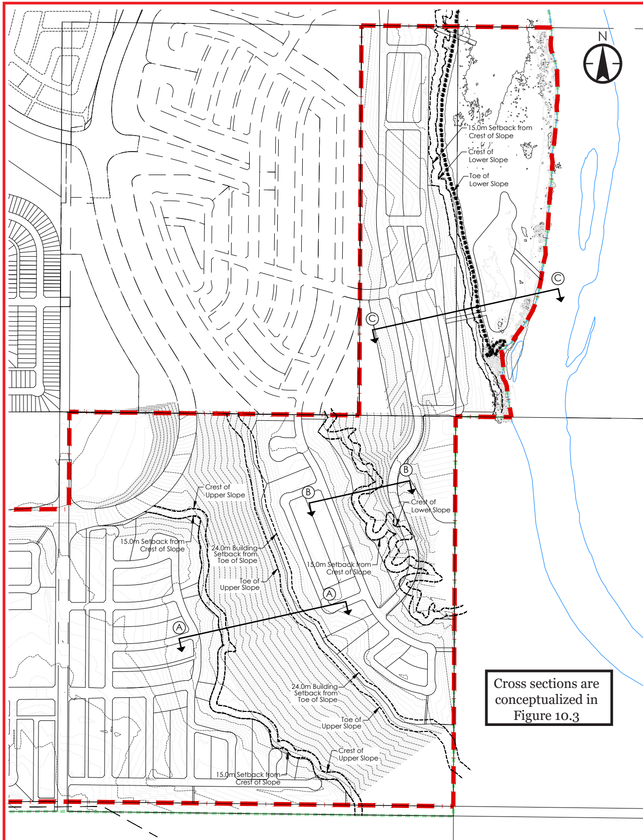
Figure 10.2 Geotechnical Setbacks
