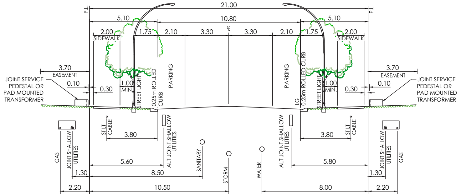
21.0m COLLECTOR PARKING BOTH SIDES / 2.0m SEPARATE WALK BOTH SIDES
