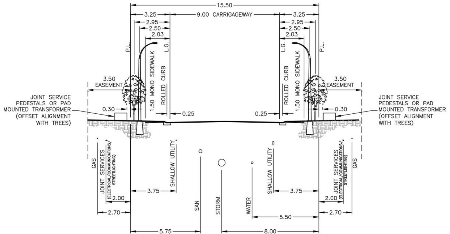
15.5m RESIDENTIAL w/ FRONT DRIVE
